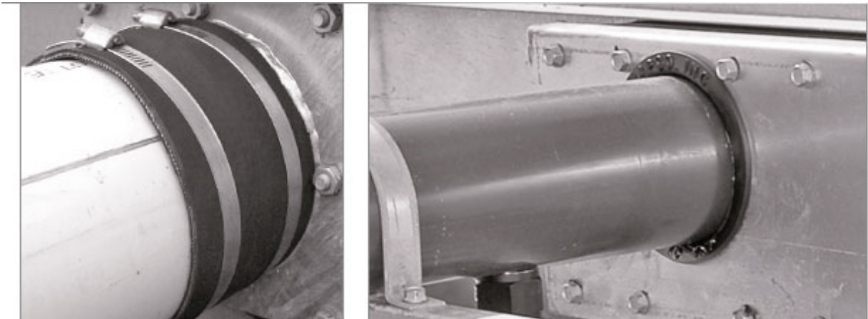
Rubber connections with straps. O-rings for distribution pipes.
